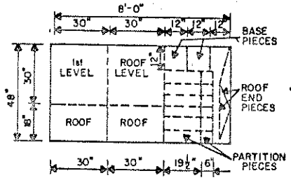
ROOF DETAILS
