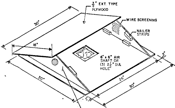
ROOF DETAILS
